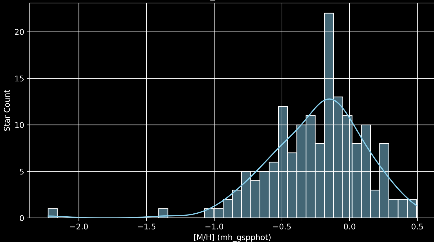
APOGEE DR17 Field: [278-21-O_TESS [M/H] (mh_gspphot) (n= 158)
