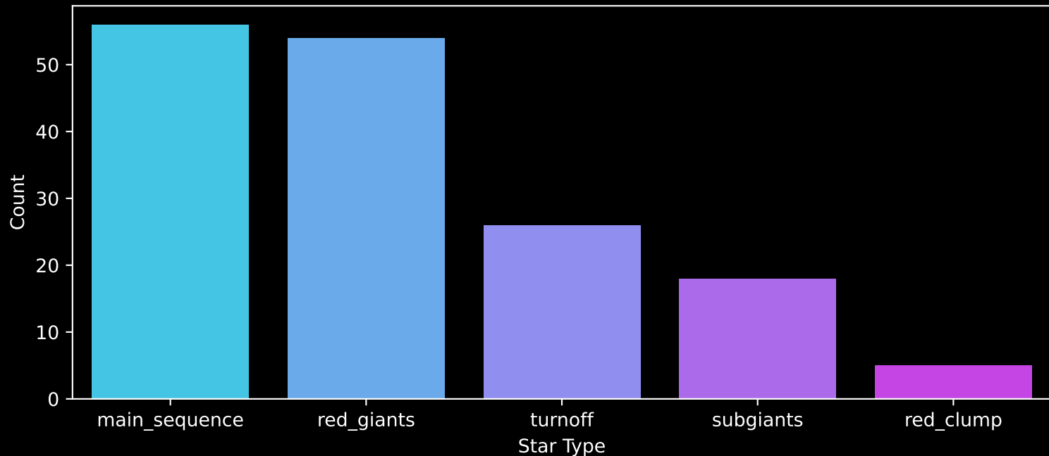
APOGEE DR17 Field: [278-21-O_TESS] Count plot of Star Type
