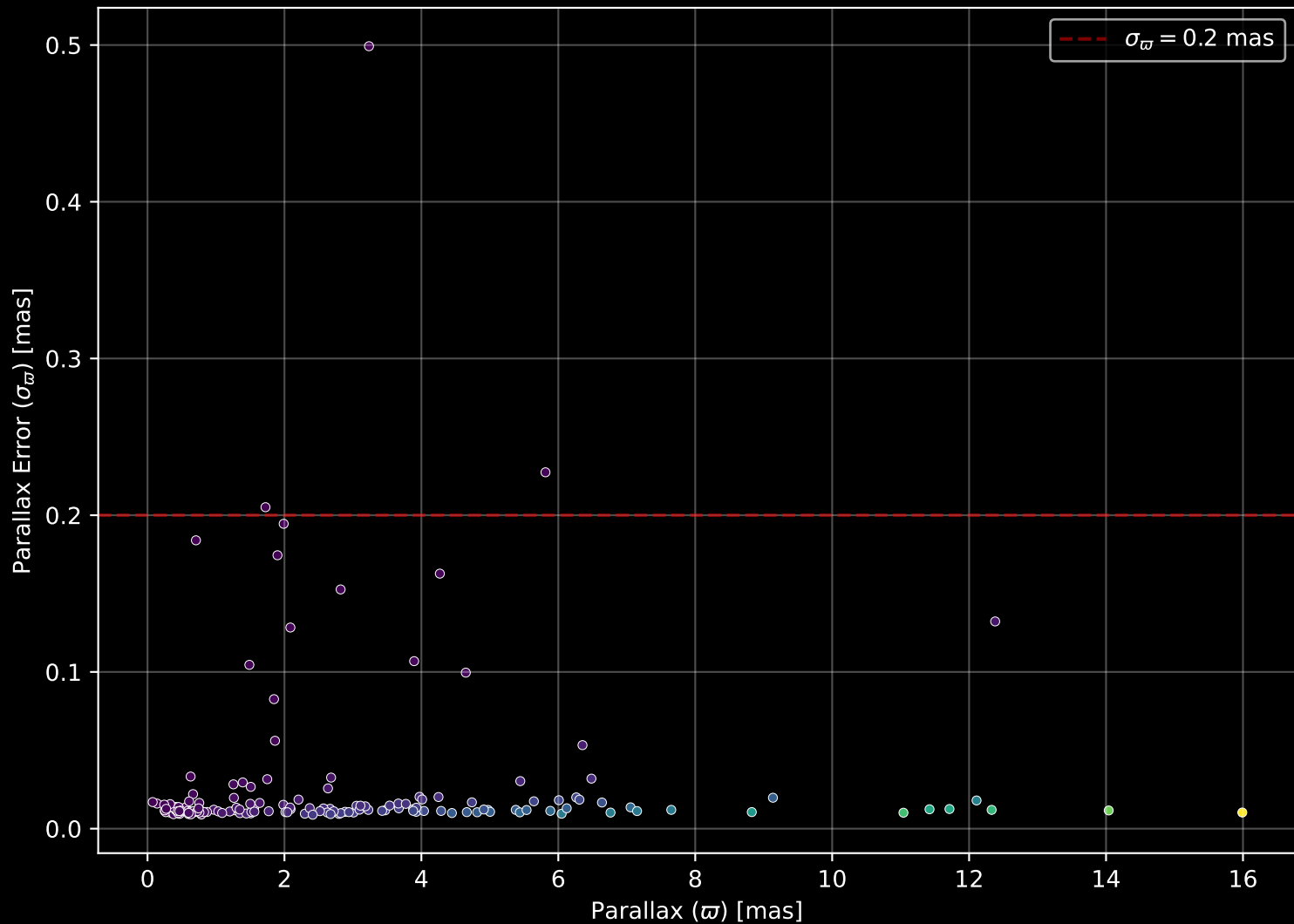
APOGEE DR17 Field: [278-21-O_TESS] Parallax Quality (n= 159)
