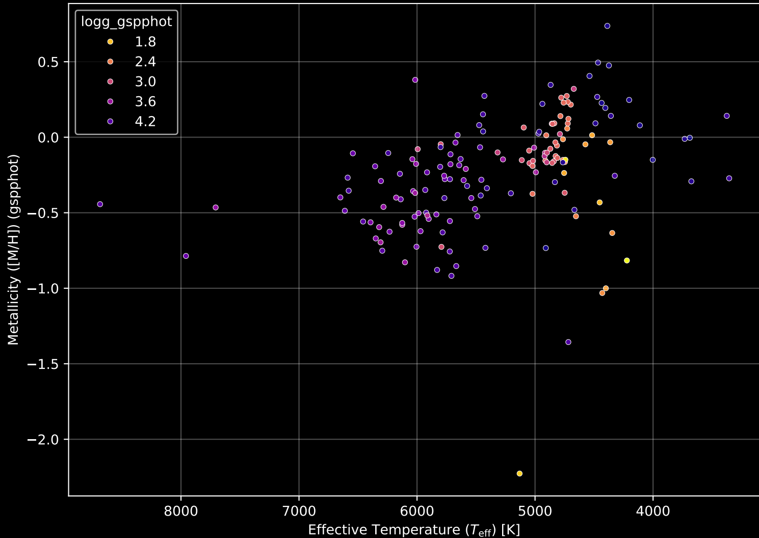
APOGEE DR17 Field: [278-21-O_TESS] Stellar Population Parameters (n= 159)
