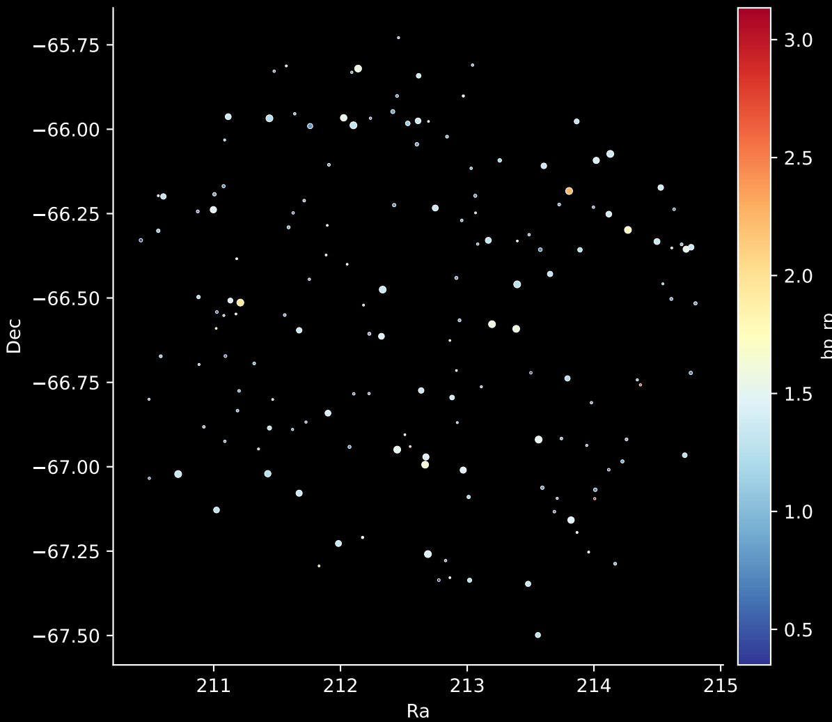
APOGEE DR17 Field: [278-21-O_TESS] Stars: 159
